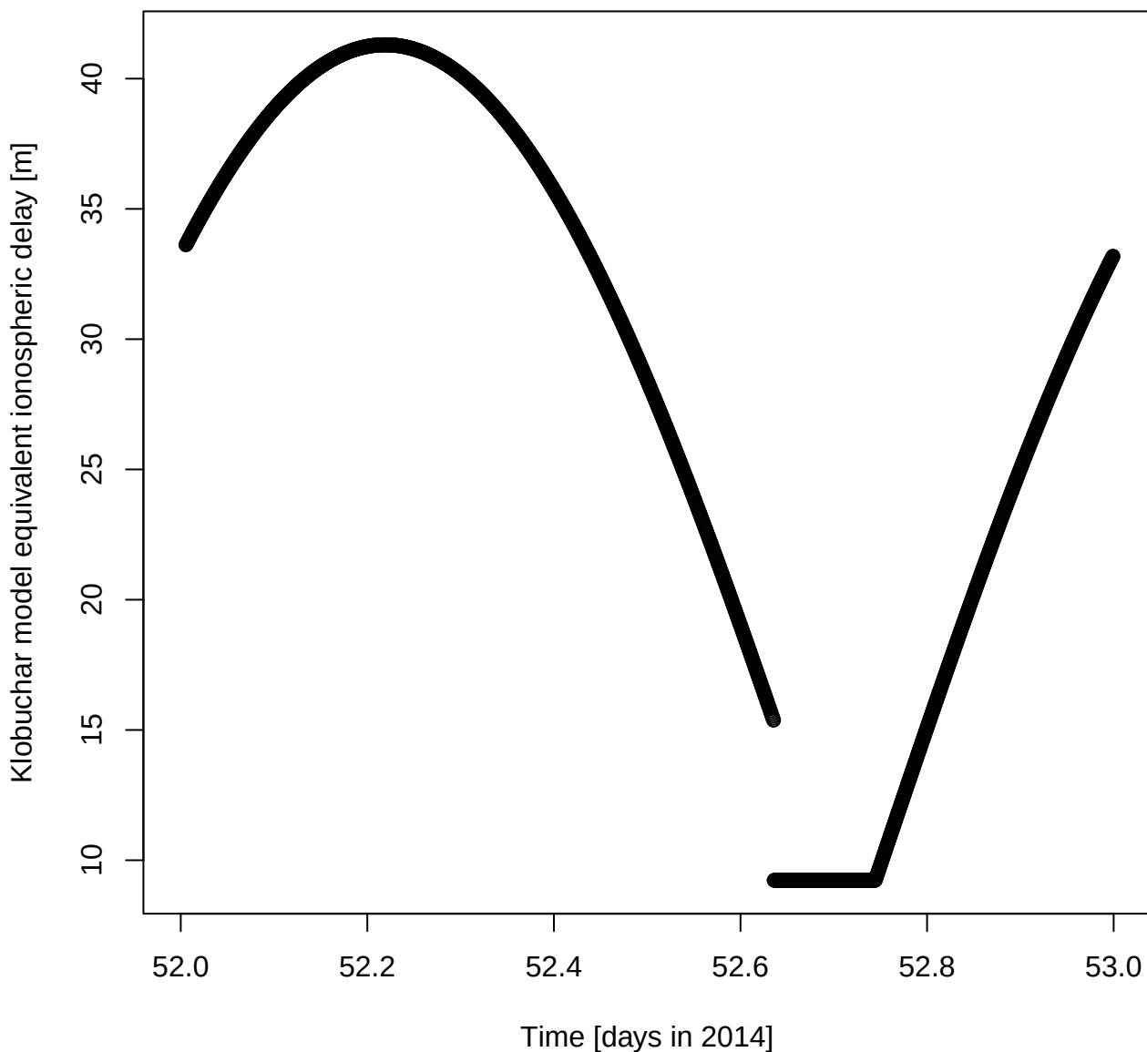
Klobuchar model equivalent ionospheric delay [m] for DOY 52 in 2014
