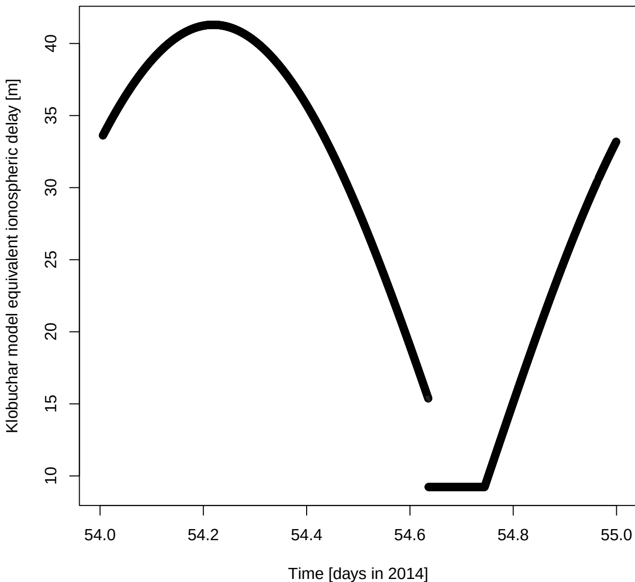
Klobuchar model equivalent ionospheric delay [m] for DOY 54 in 2014
