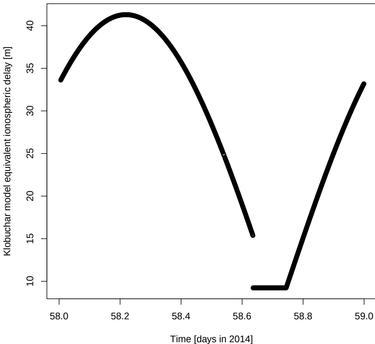
Klobuchar model equivalent ionospheric delay [m] for DOY 58 in 2014
