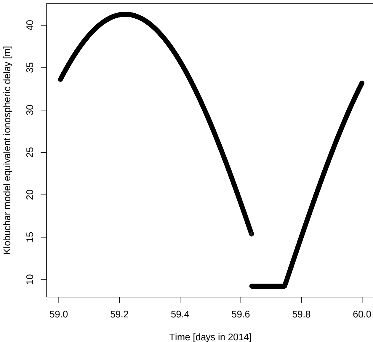
Klobuchar model equivalent ionospheric delay [m] for DOY 59 in 2014
