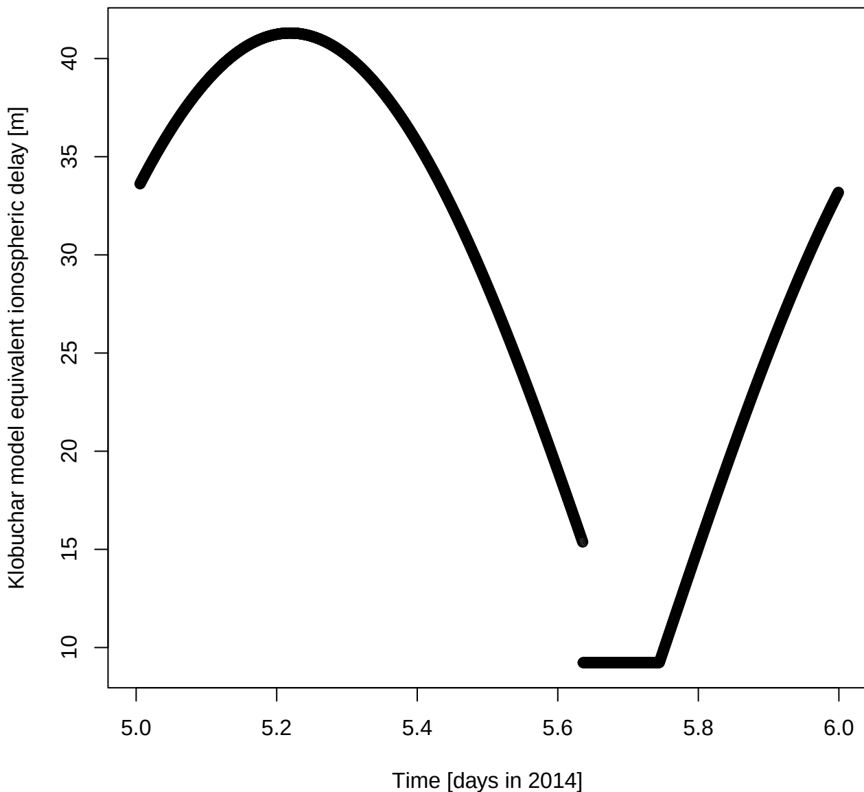
Klobuchar model equivalent ionospheric delay [m] for DOY 5 in 2014
