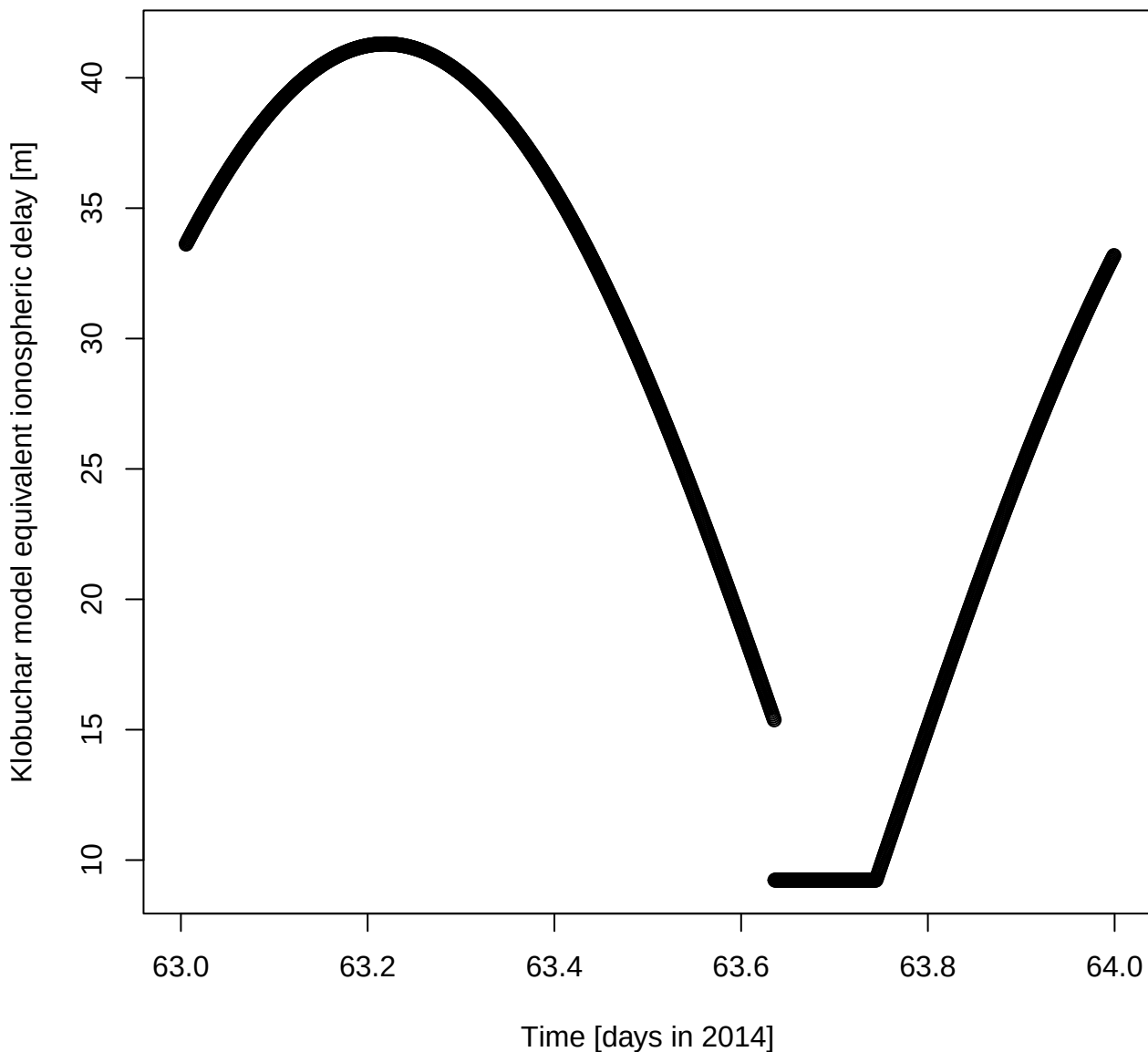
Klobuchar model equivalent ionospheric delay [m] for DOY 63 in 2014
