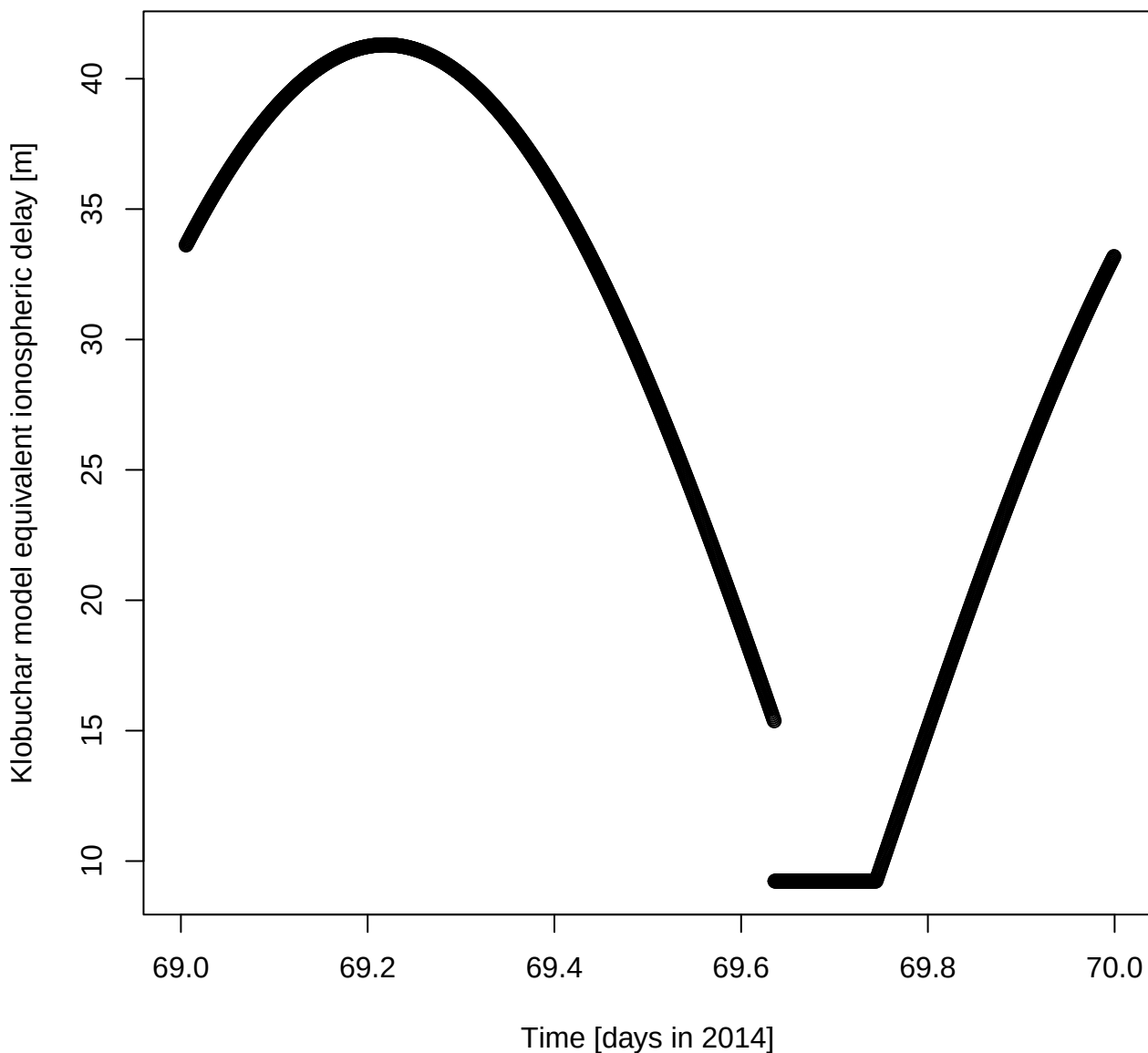
Klobuchar model equivalent ionospheric delay [m] for DOY 69 in 2014
