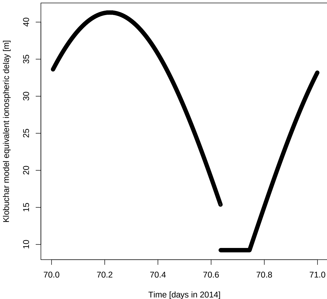
Klobuchar model equivalent ionospheric delay [m] for DOY 70 in 2014
