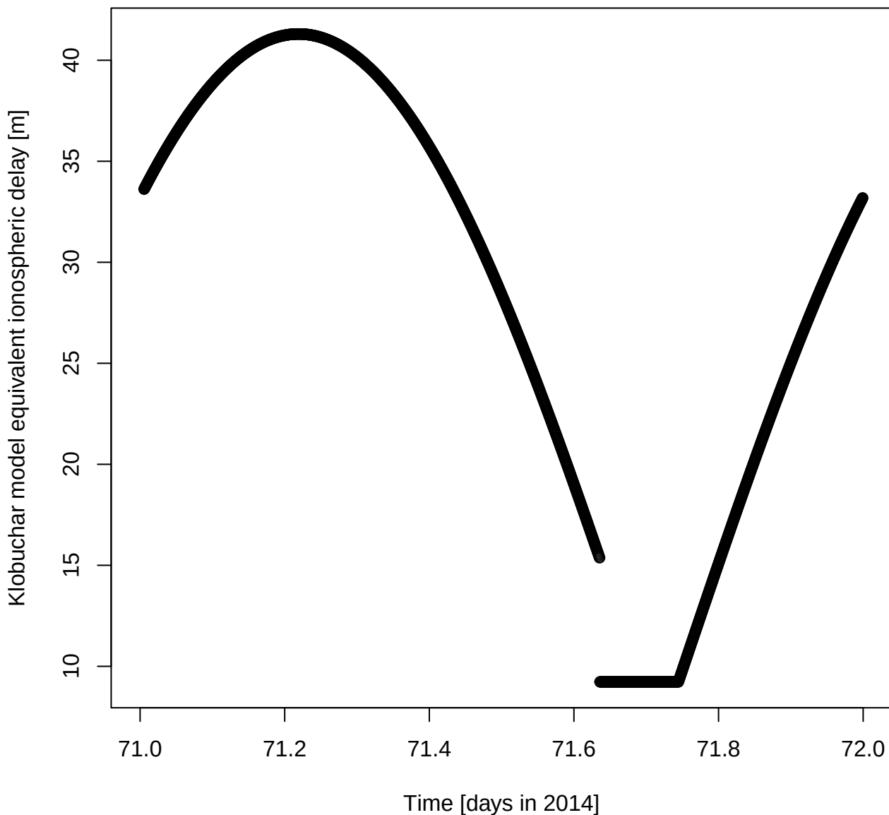
Klobuchar model equivalent ionospheric delay [m] for DOY 71 in 2014
