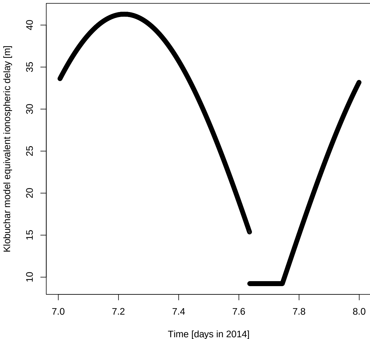
Klobuchar model equivalent ionospheric delay [m] for DOY 7 in 2014
