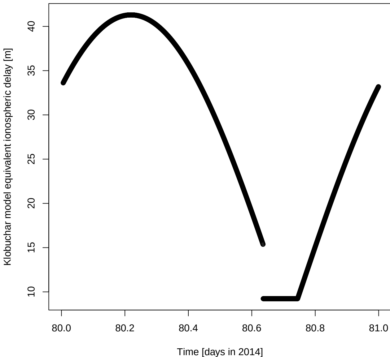
Klobuchar model equivalent ionospheric delay [m] for DOY 80 in 2014
