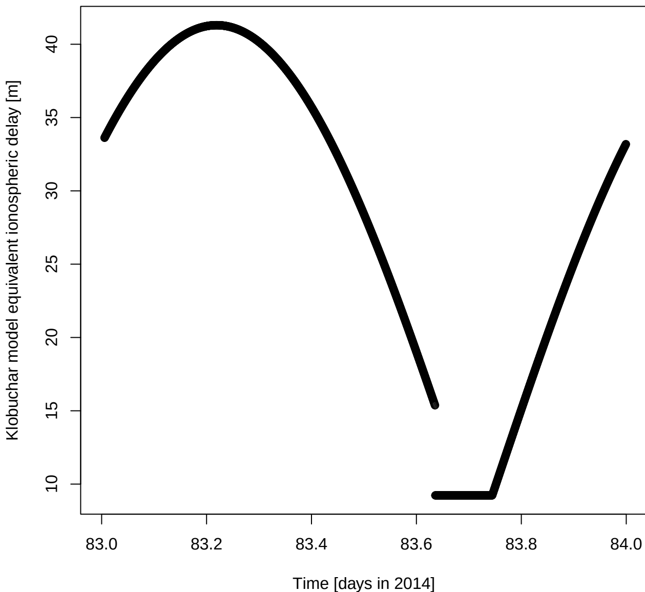
Klobuchar model equivalent ionospheric delay [m] for DOY 83 in 2014
