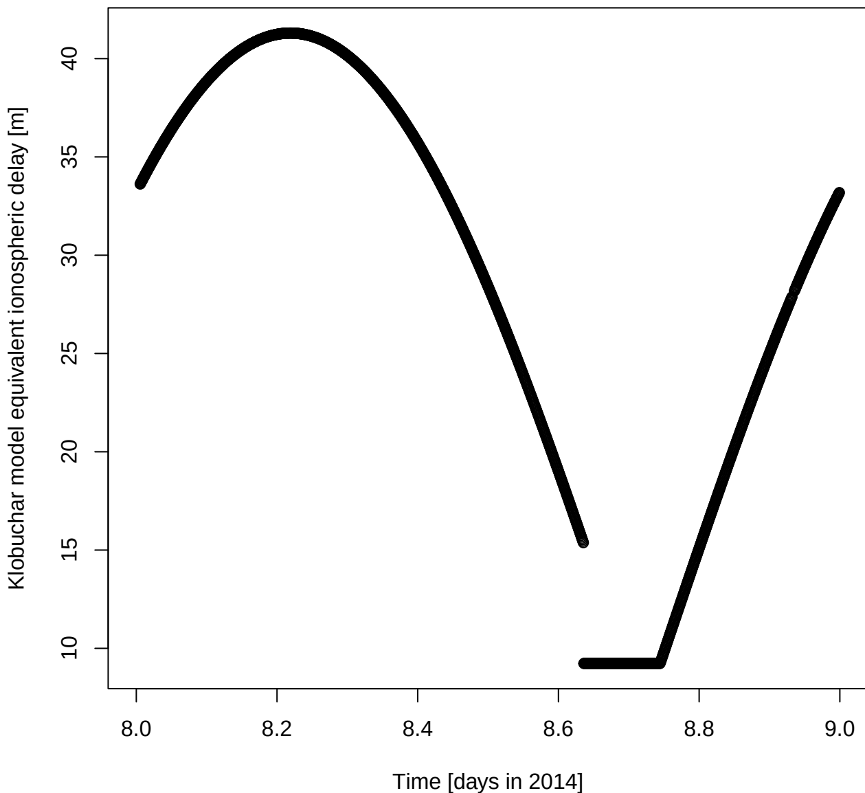
Klobuchar model equivalent ionospheric delay [m] for DOY 8 in 2014
