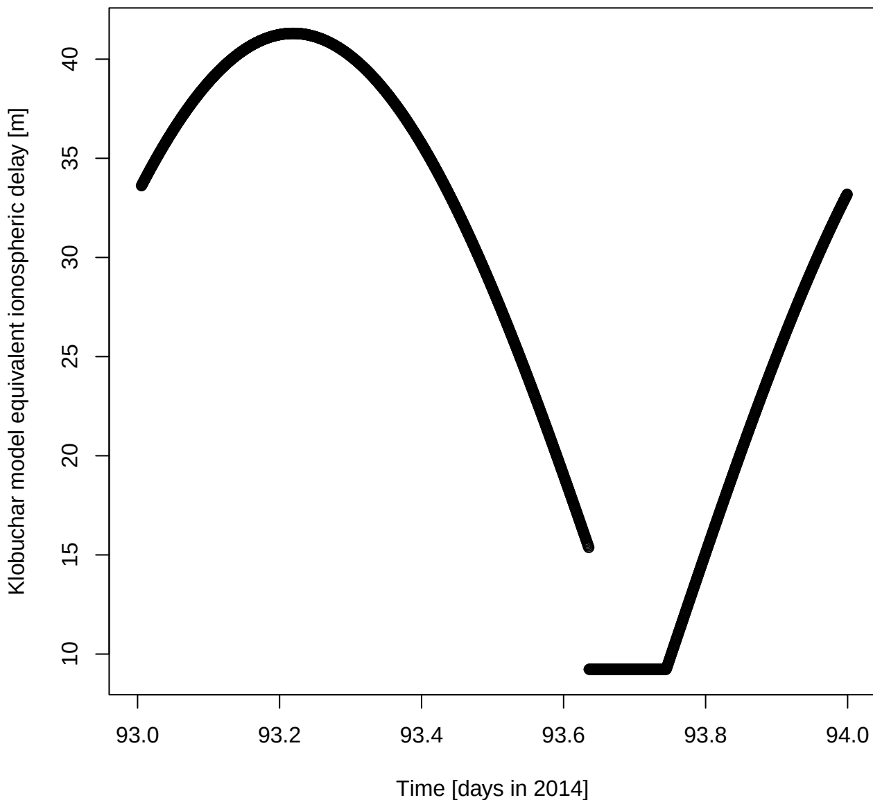
Klobuchar model equivalent ionospheric delay [m] for DOY 93 in 2014
