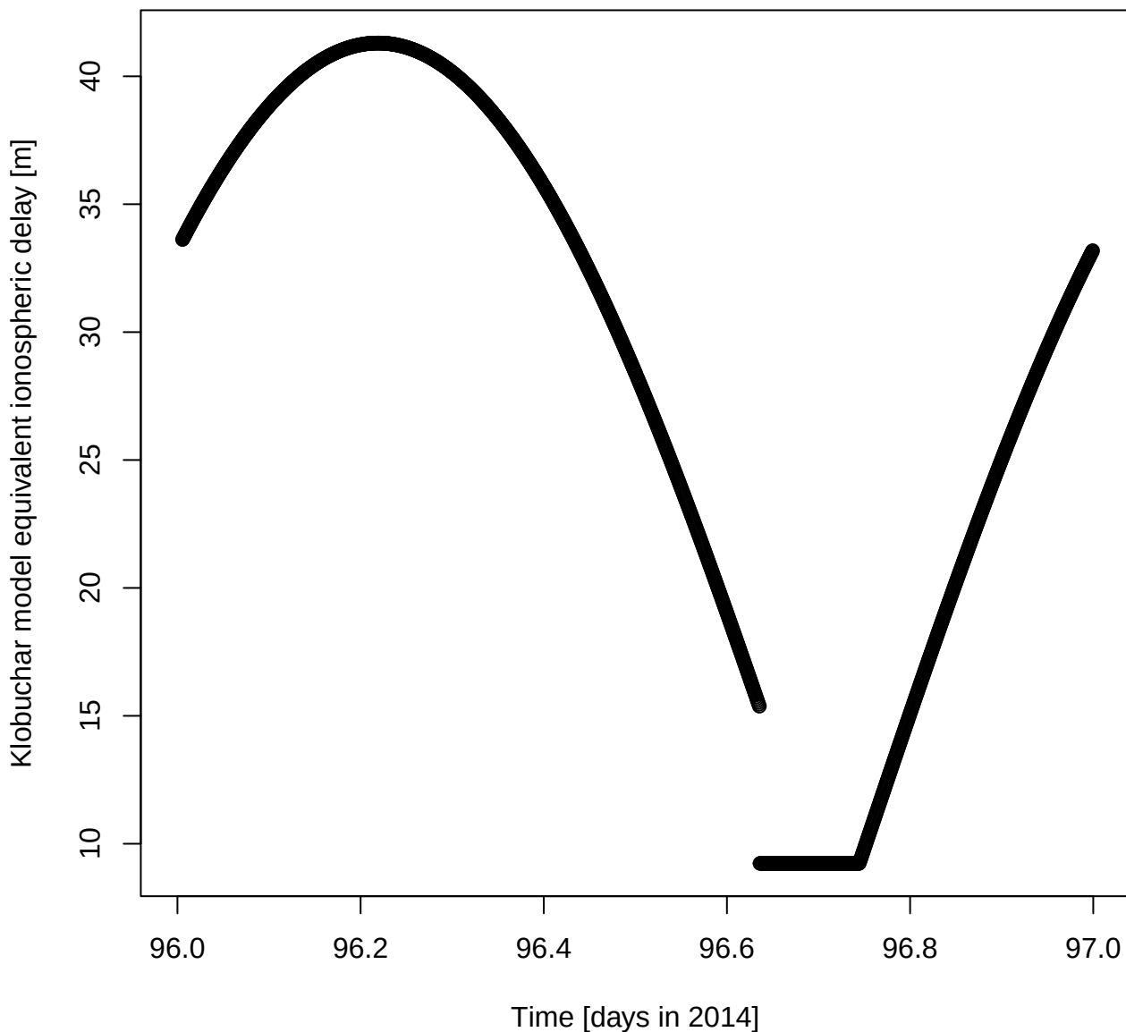
Klobuchar model equivalent ionospheric delay [m] for DOY 96 in 2014
