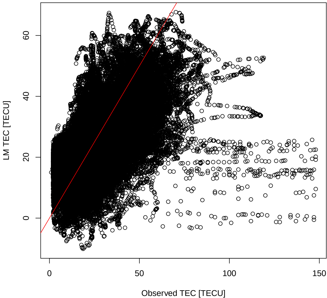
Observed and LM-predicted TEC [TECU]
