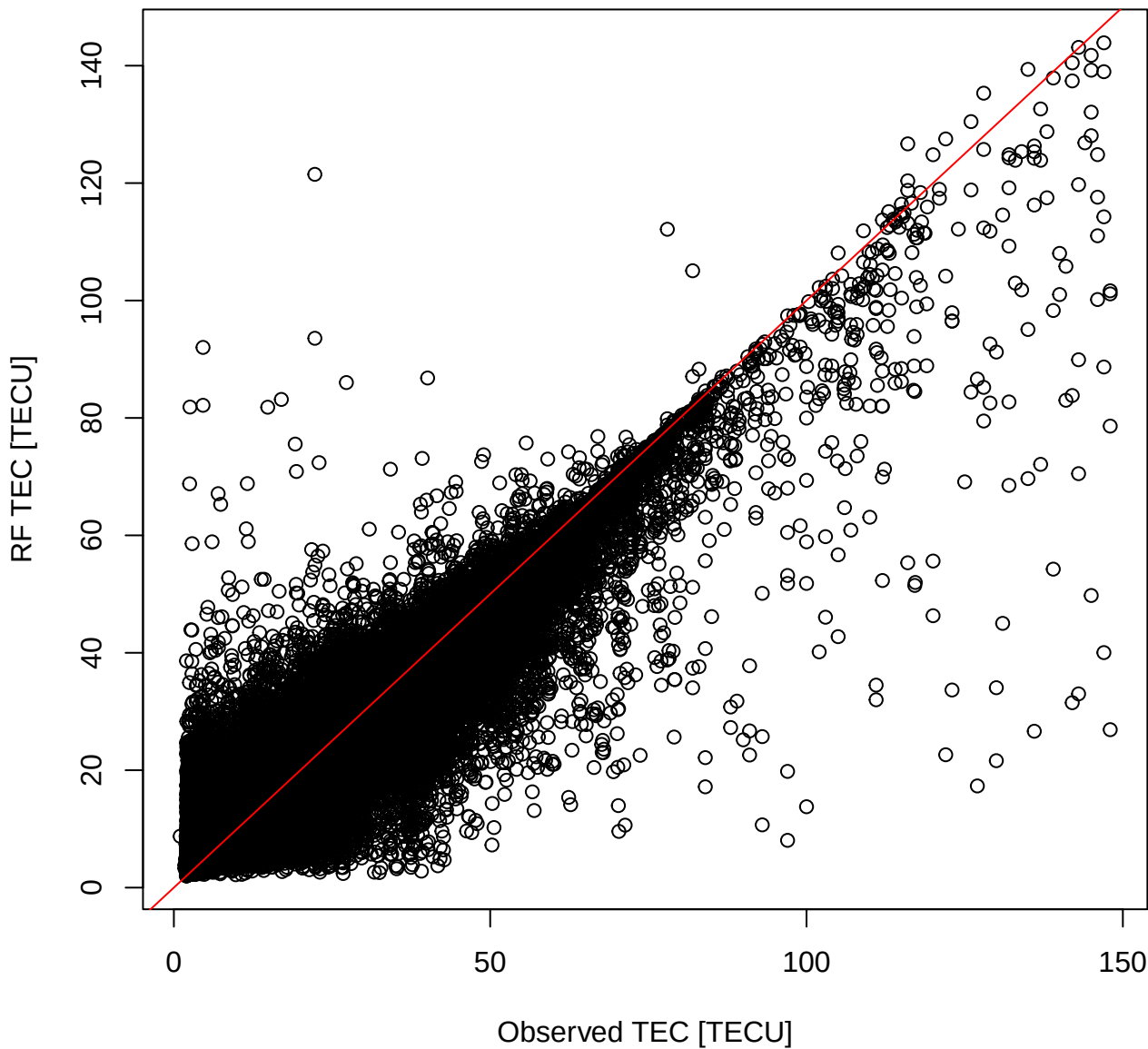
Observed and RF-predicted TEC [TECU]
