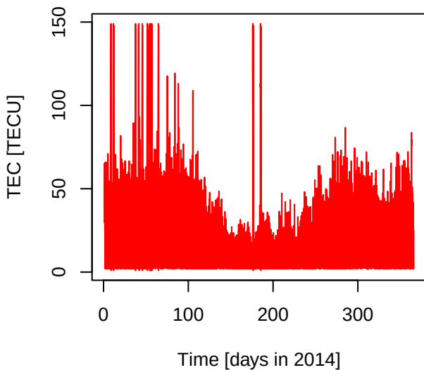
TEC [TECU] for days in 2014
