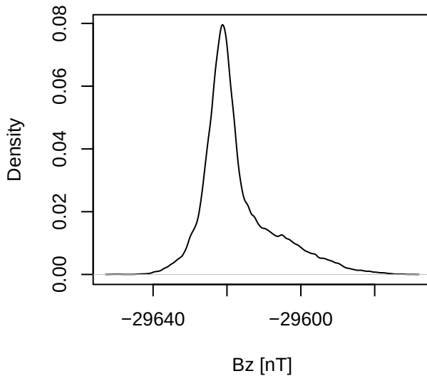
Probability density Bz [nT]
