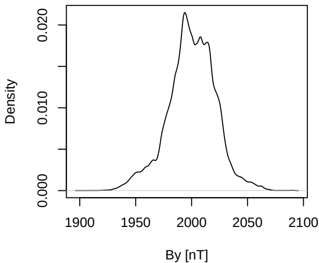
Probability density By [nT]
