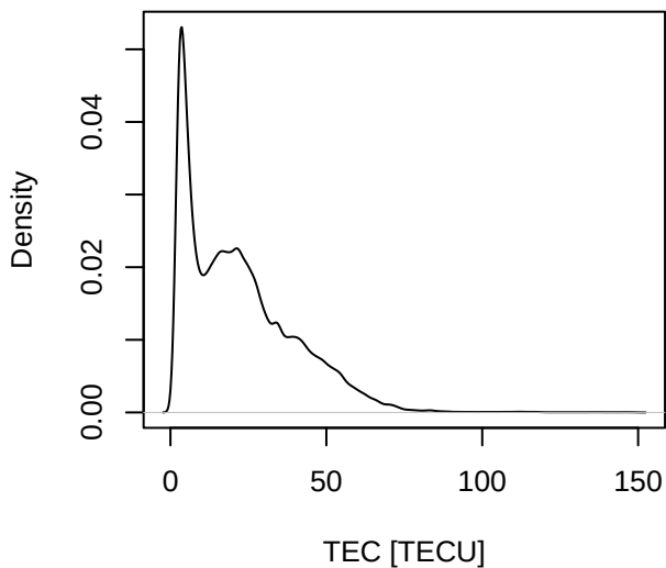
Probability density TEC [TECU]
