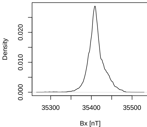
Probability density Bx [nT]
