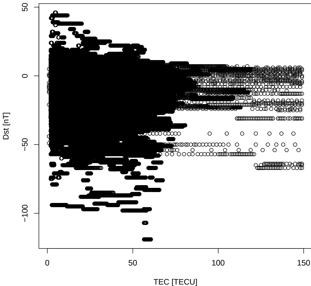
TEC [TECU] and Dst [nT] for days in 2014
