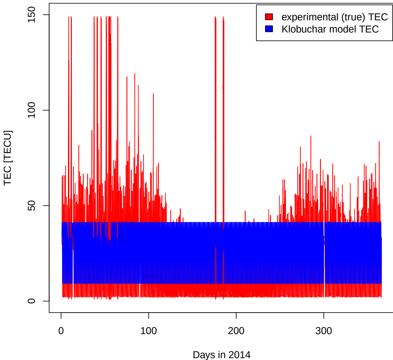
Klobuchar model and experimental (true) TEC in 2014
