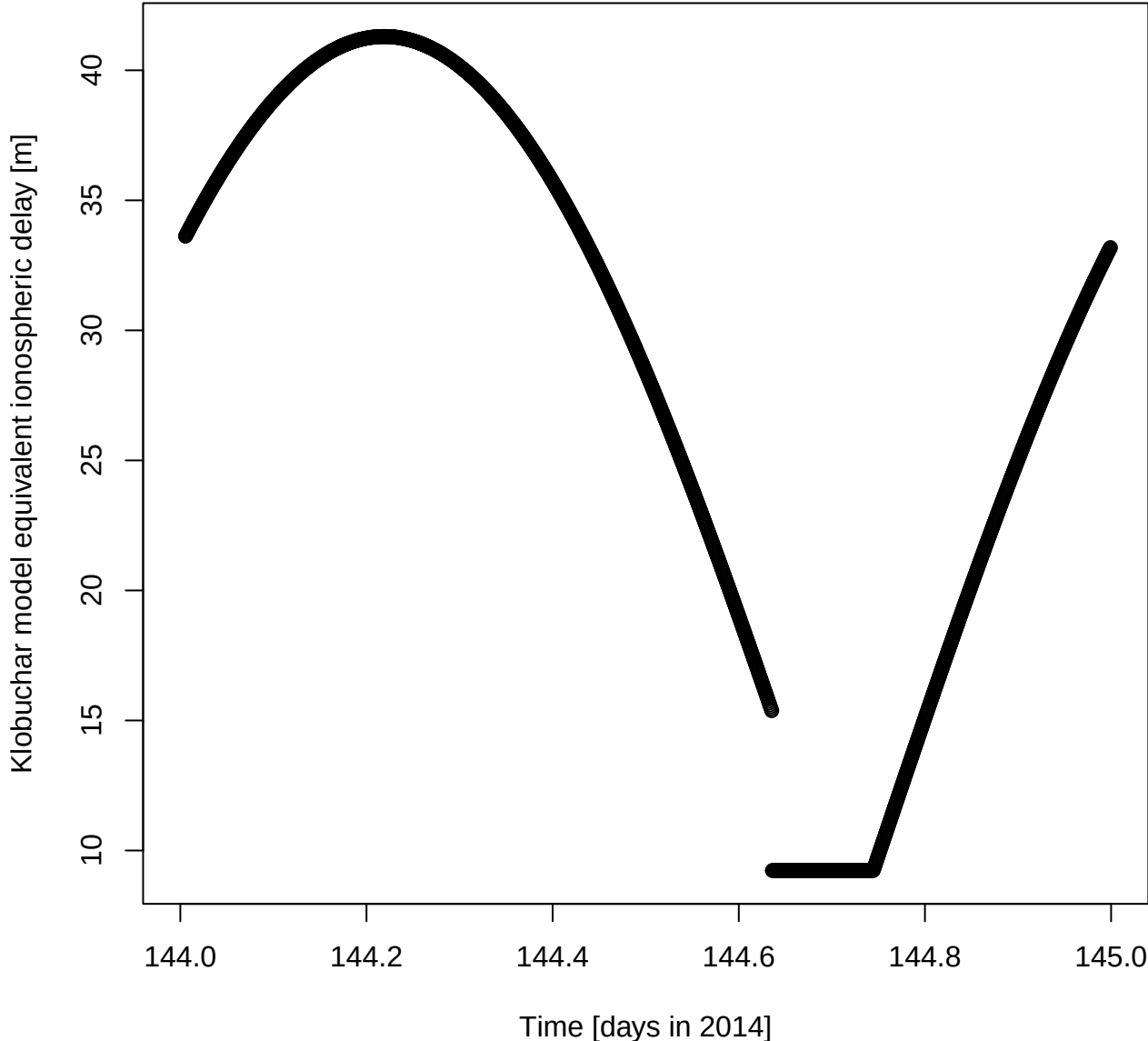
Klobuchar model equivalent ionospheric delay [m] for DOY 144 in 2014
