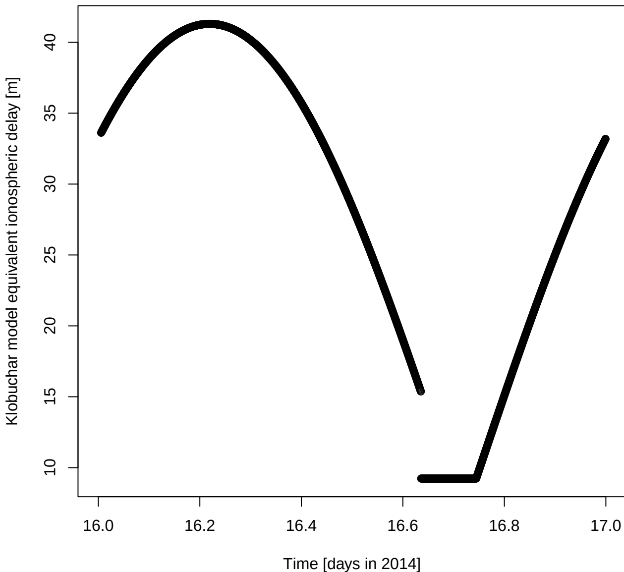
Klobuchar model equivalent ionospheric delay [m] for DOY 16 in 2014
