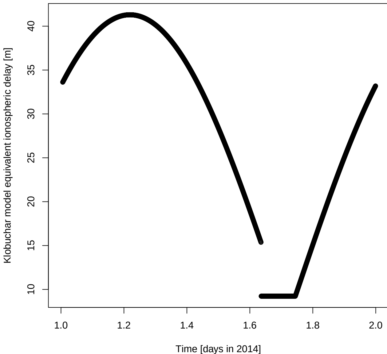
Klobuchar model equivalent ionospheric delay [m] for DOY 1 in 2014
