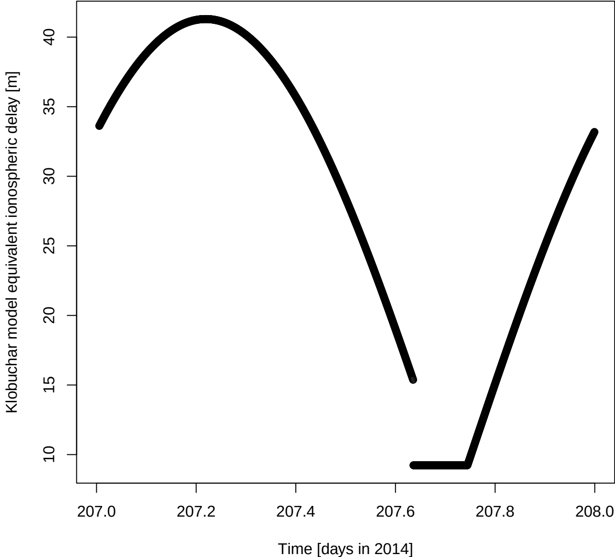
Klobuchar model equivalent ionospheric delay [m] for DOY 207 in 2014
