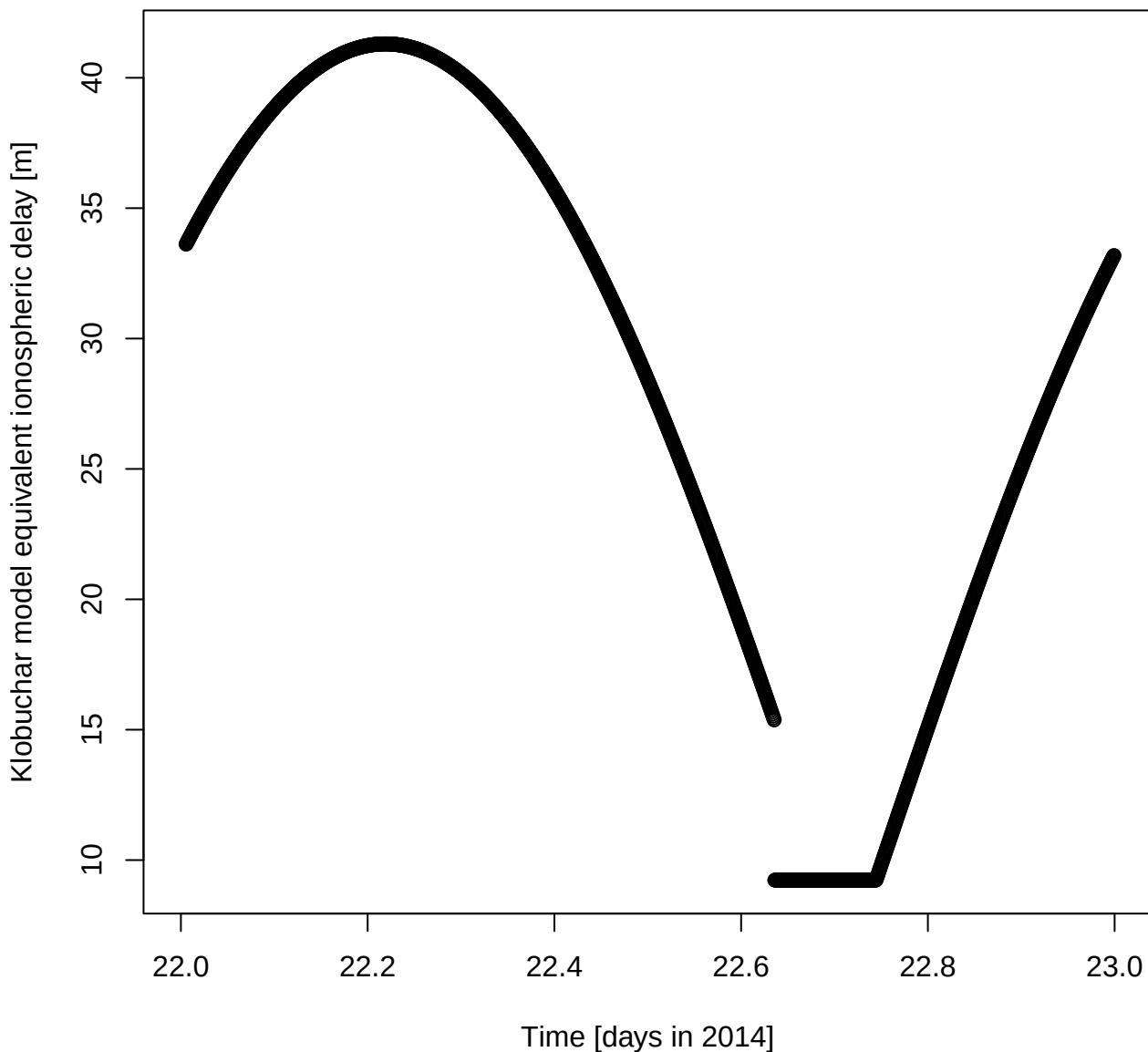
Klobuchar model equivalent ionospheric delay [m] for DOY 22 in 2014
