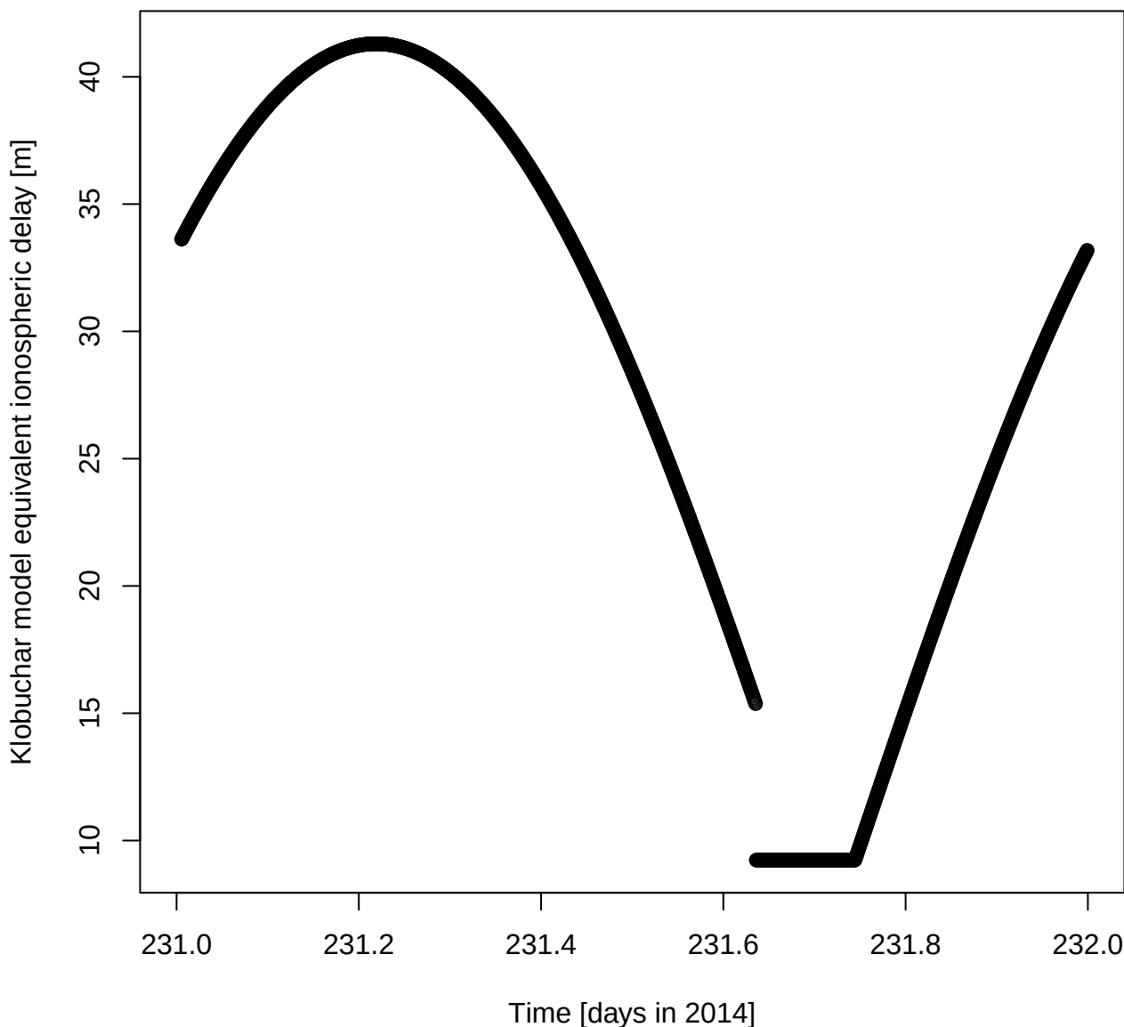
Klobuchar model equivalent ionospheric delay [m] for DOY 231 in 2014
