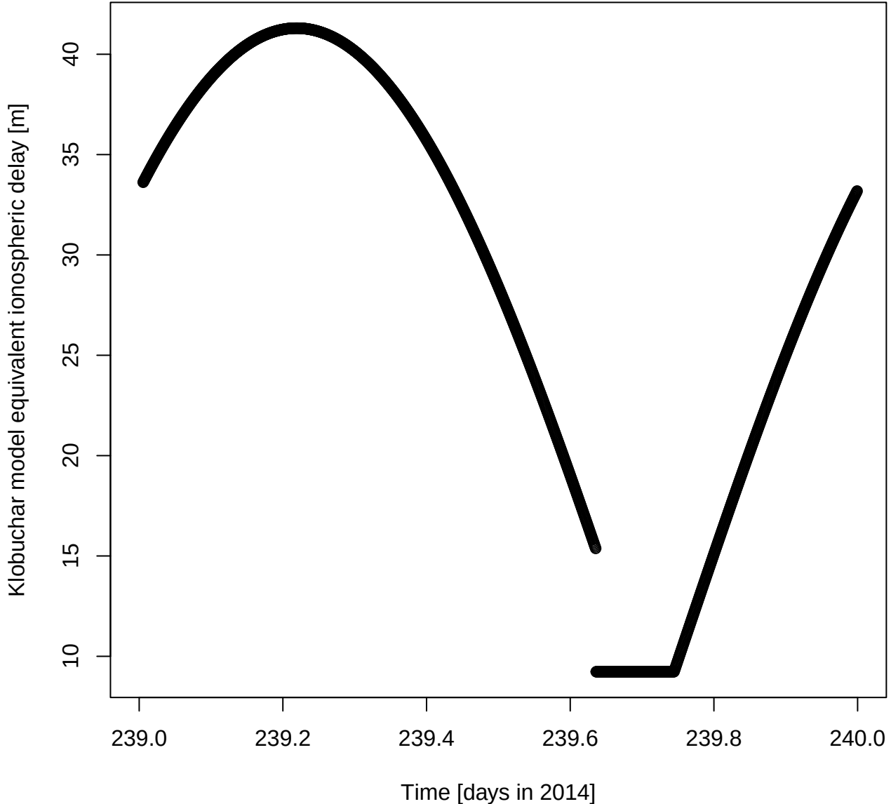
Klobuchar model equivalent ionospheric delay [m] for DOY 239 in 2014
