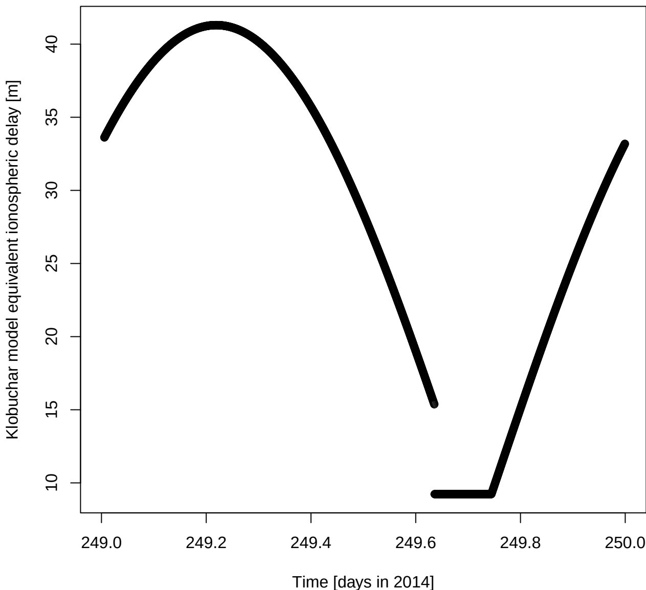
Klobuchar model equivalent ionospheric delay [m] for DOY 249 in 2014
