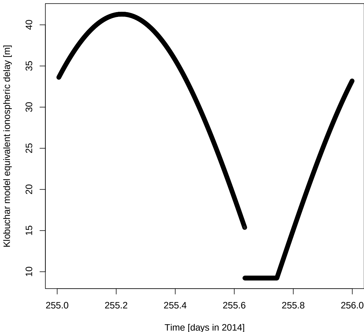
Klobuchar model equivalent ionospheric delay [m] for DOY 255 in 2014
