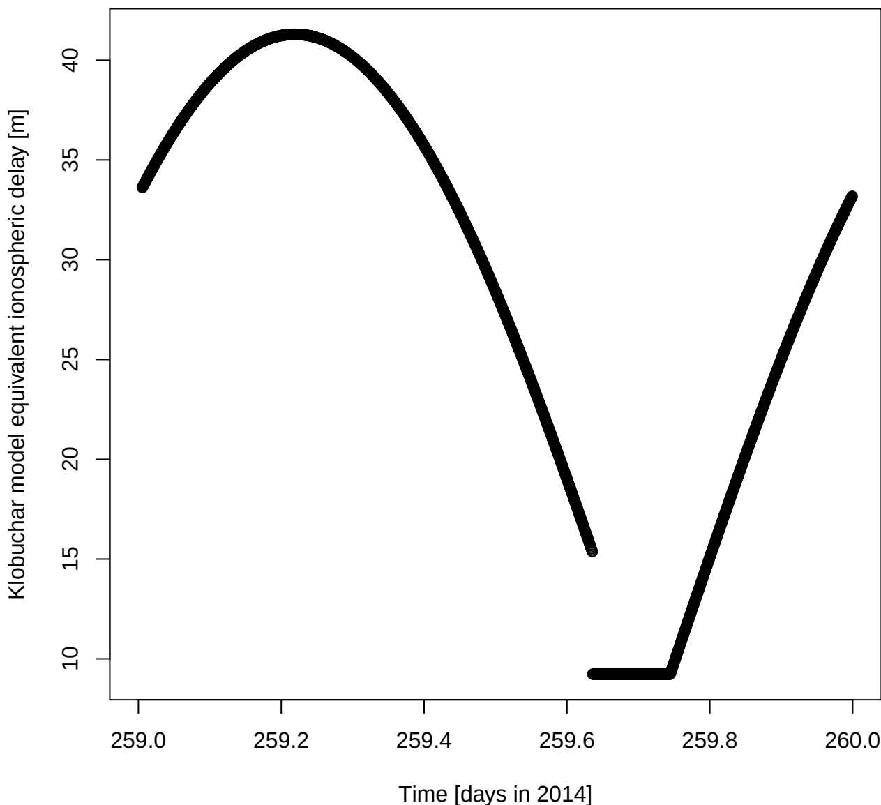
Klobuchar model equivalent ionospheric delay [m] for DOY 259 in 2014
