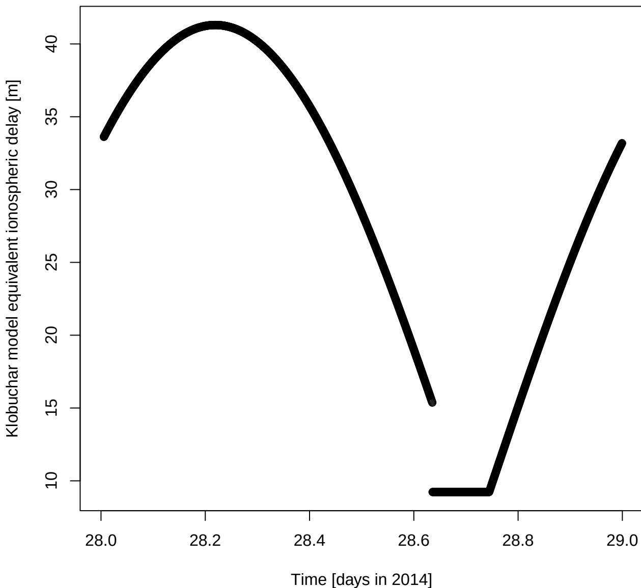
Klobuchar model equivalent ionospheric delay [m] for DOY 28 in 2014
