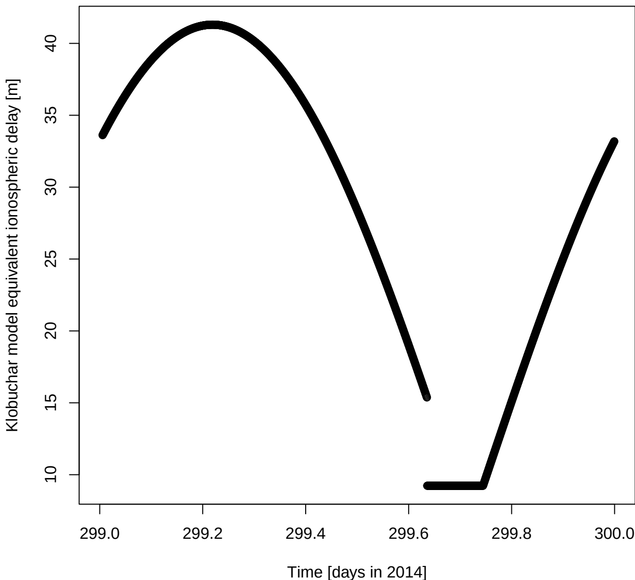
Klobuchar model equivalent ionospheric delay [m] for DOY 299 in 2014
