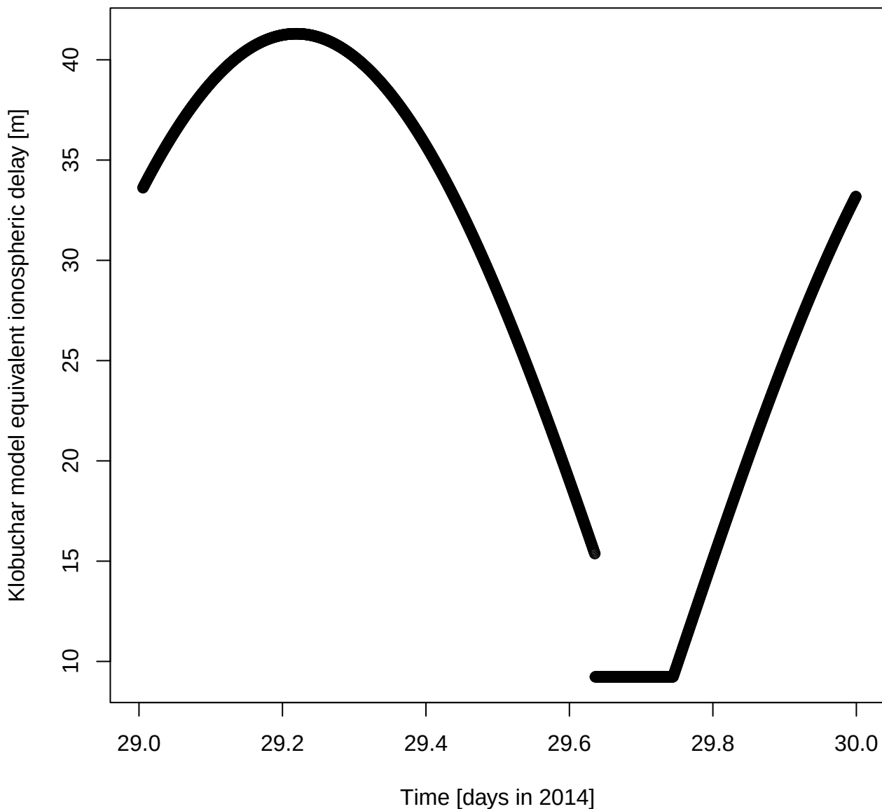
Klobuchar model equivalent ionospheric delay [m] for DOY 29 in 2014
