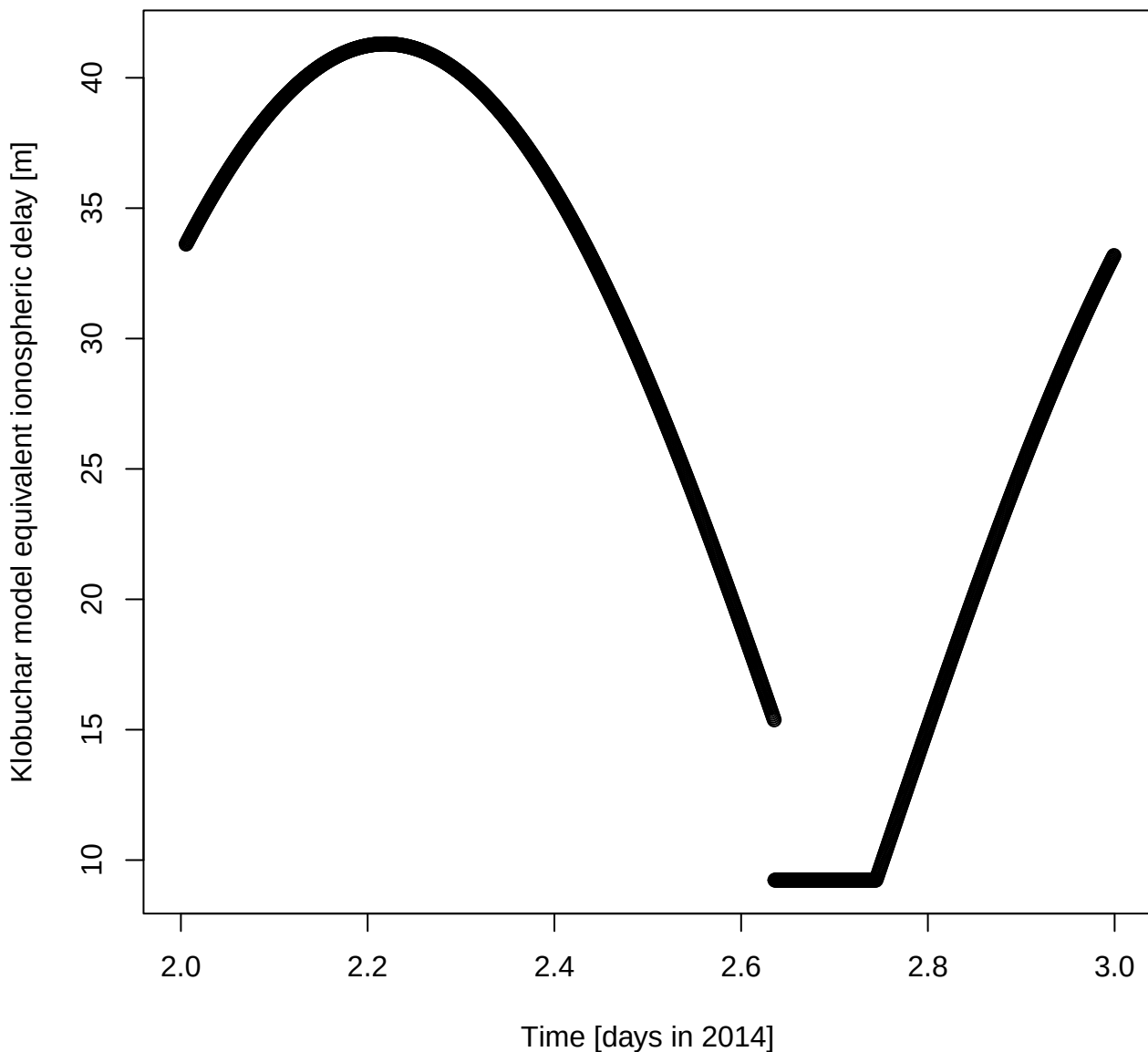
Klobuchar model equivalent ionospheric delay [m] for DOY 2 in 2014
