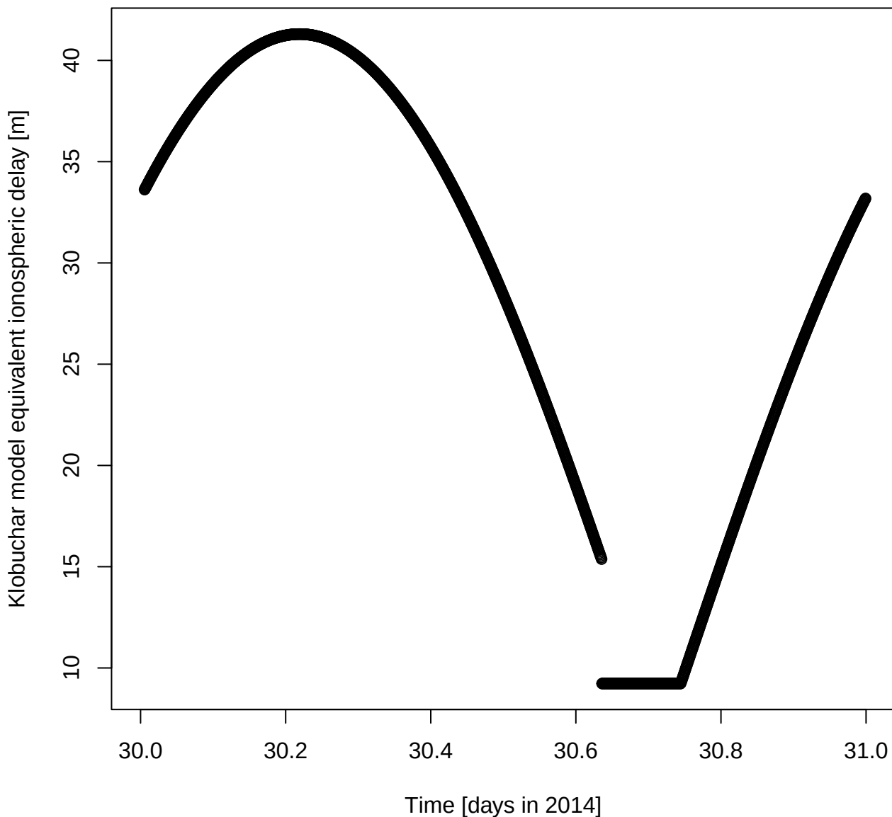
Klobuchar model equivalent ionospheric delay [m] for DOY 30 in 2014
