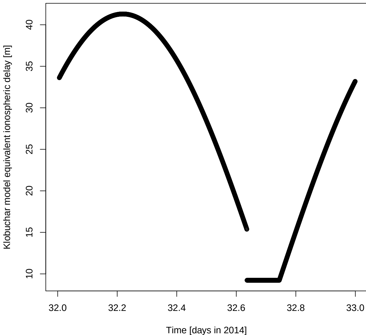
Klobuchar model equivalent ionospheric delay [m] for DOY 32 in 2014
