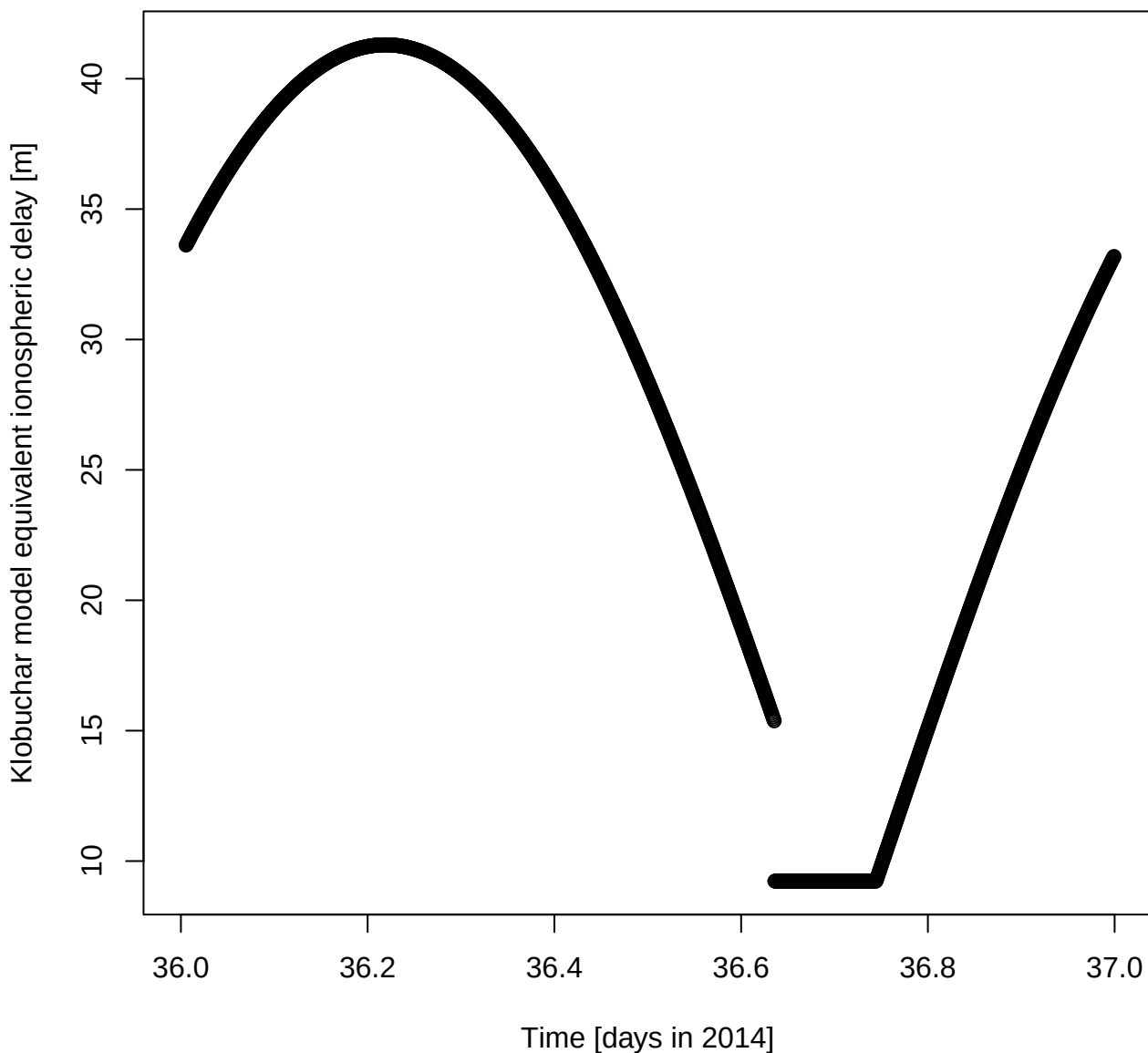
Klobuchar model equivalent ionospheric delay [m] for DOY 36 in 2014
