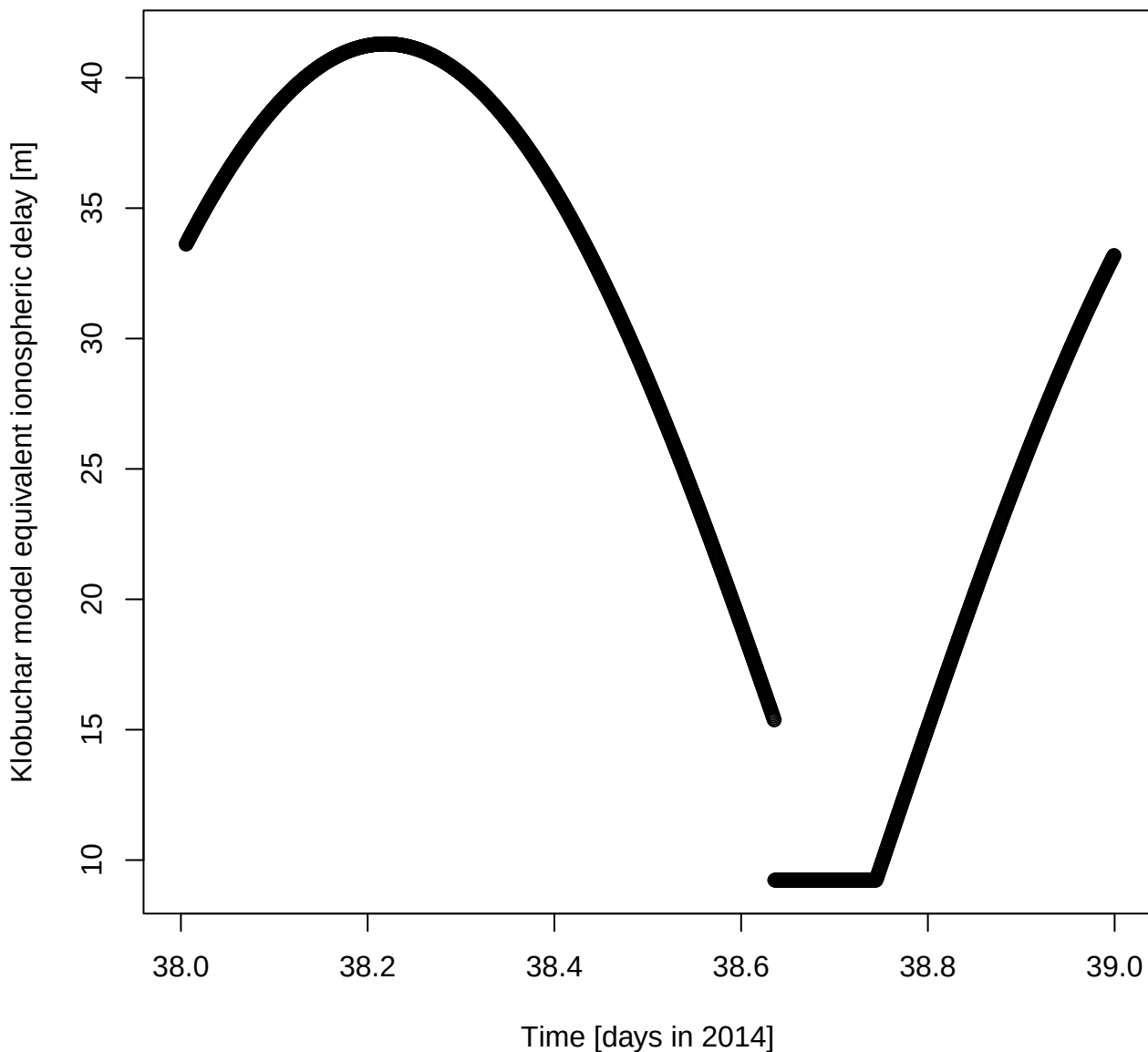
Klobuchar model equivalent ionospheric delay [m] for DOY 38 in 2014
