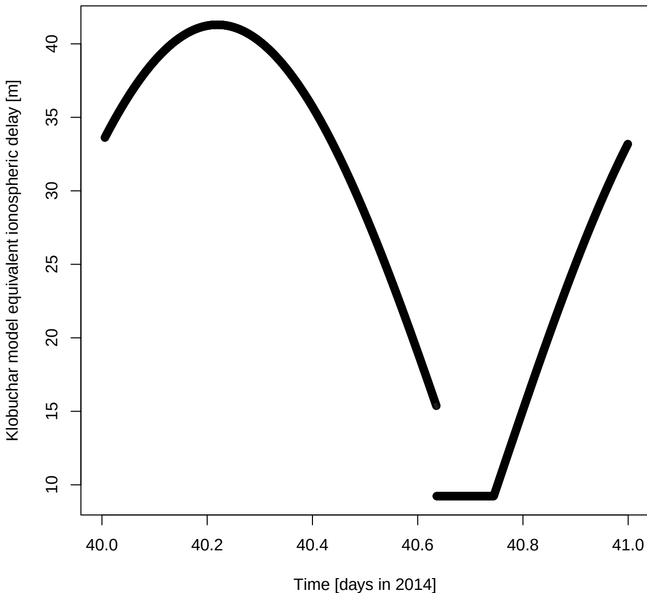
Klobuchar model equivalent ionospheric delay [m] for DOY 40 in 2014
