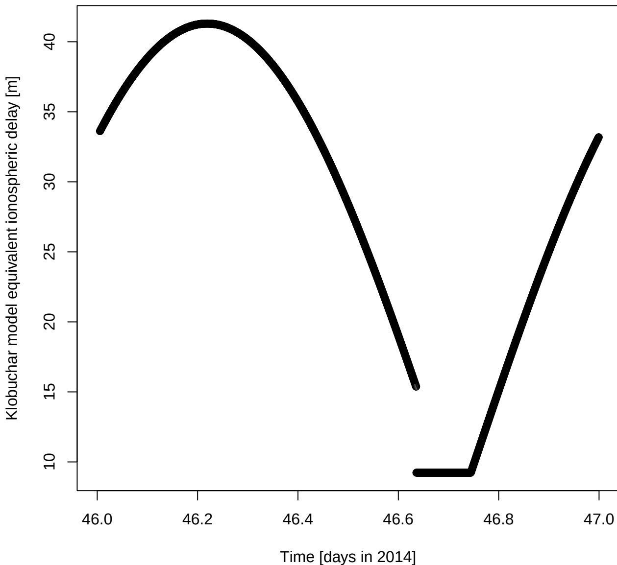
Klobuchar model equivalent ionospheric delay [m] for DOY 46 in 2014
