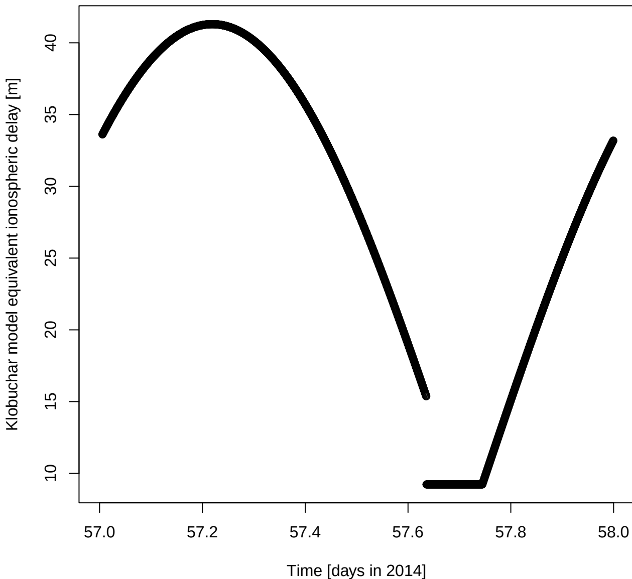
Klobuchar model equivalent ionospheric delay [m] for DOY 57 in 2014
