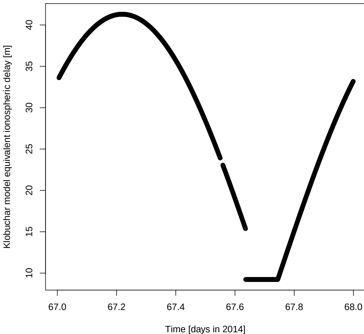
Klobuchar model equivalent ionospheric delay [m] for DOY 67 in 2014
