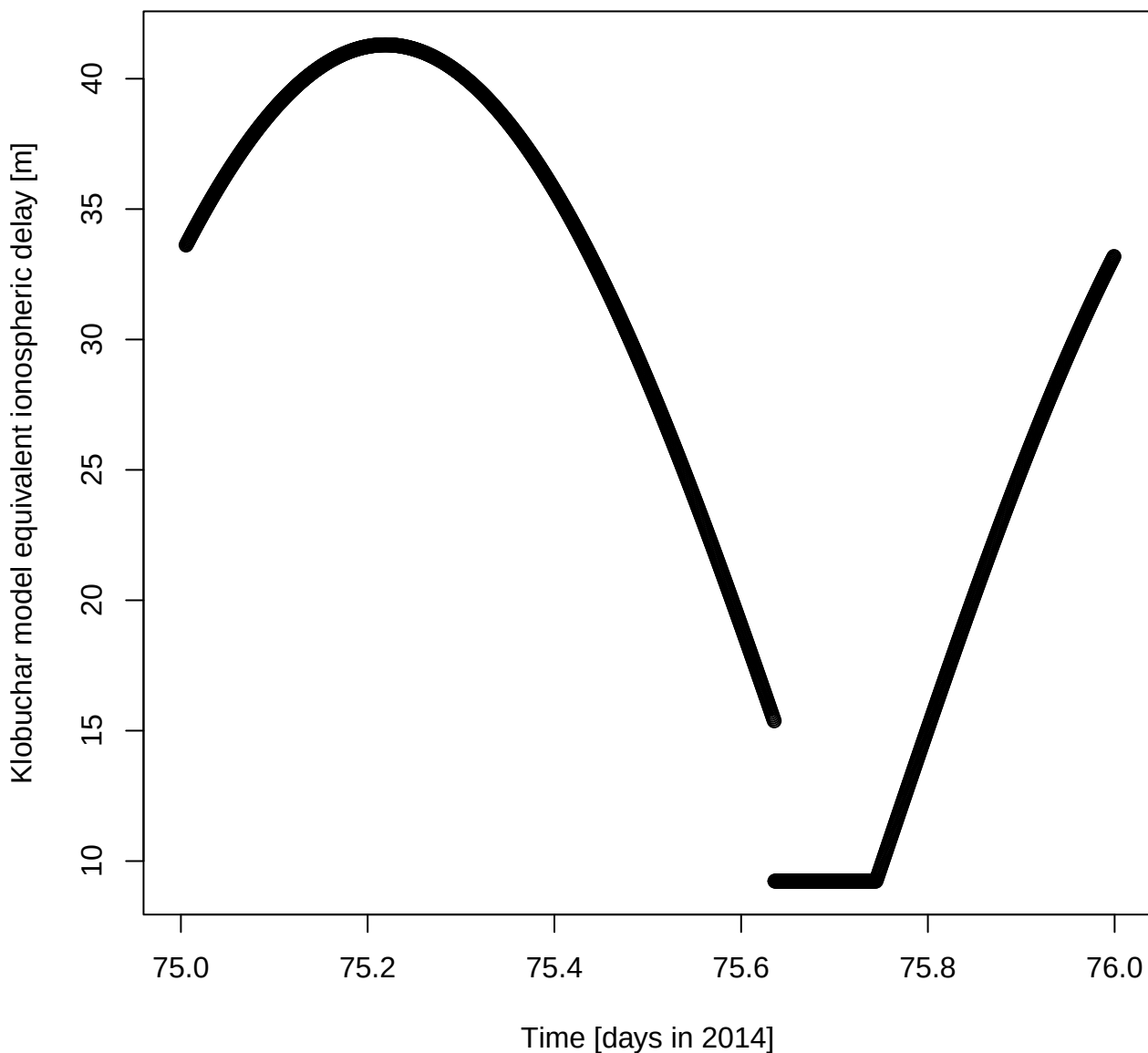
Klobuchar model equivalent ionospheric delay [m] for DOY 75 in 2014
