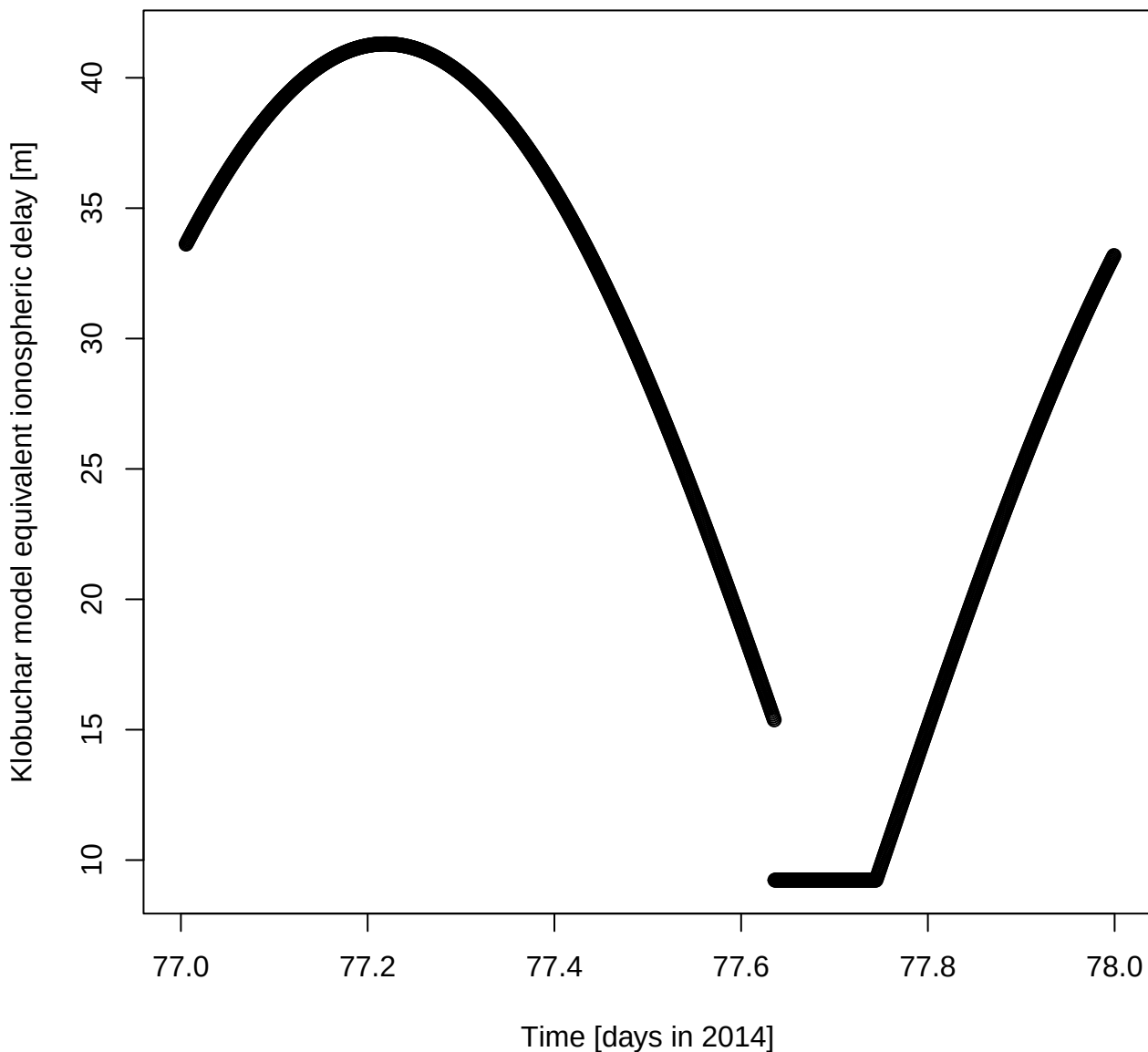
Klobuchar model equivalent ionospheric delay [m] for DOY 77 in 2014
