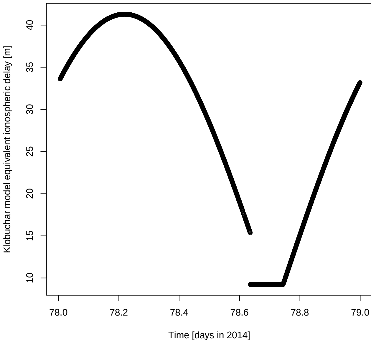
Klobuchar model equivalent ionospheric delay [m] for DOY 78 in 2014
