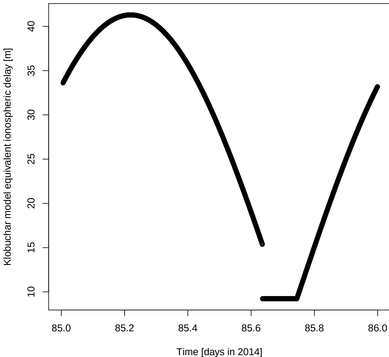
Klobuchar model equivalent ionospheric delay [m] for DOY 85 in 2014
