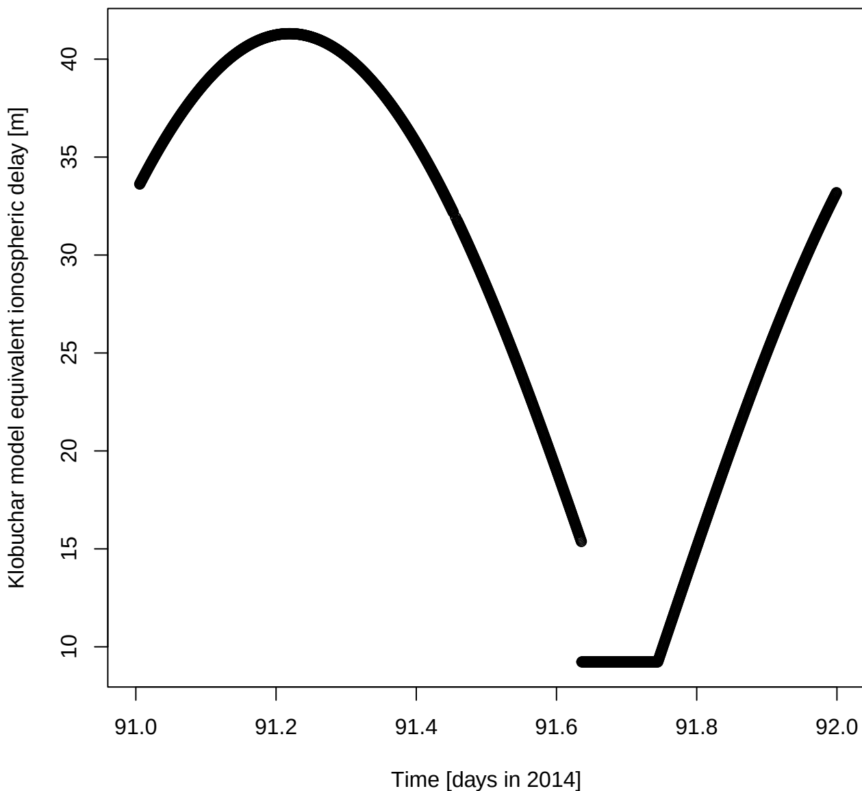
Klobuchar model equivalent ionospheric delay [m] for DOY 91 in 2014
