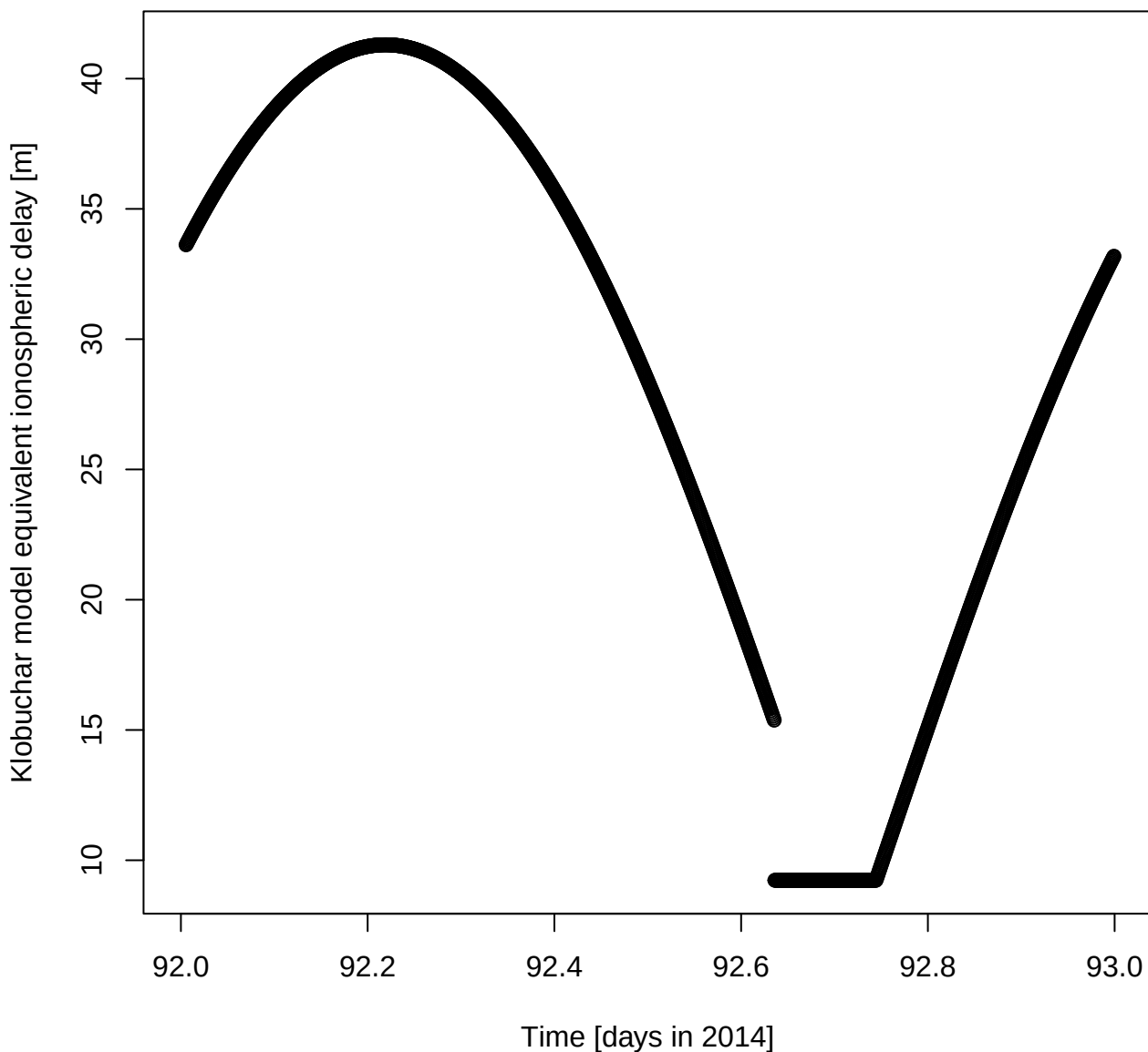
Klobuchar model equivalent ionospheric delay [m] for DOY 92 in 2014
