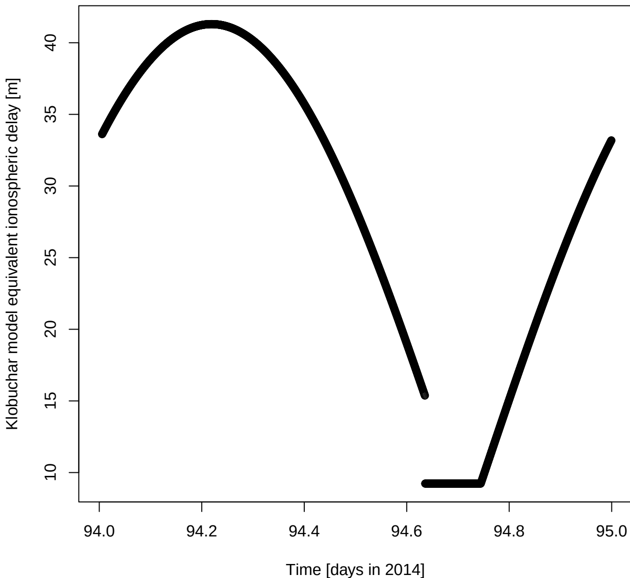
Klobuchar model equivalent ionospheric delay [m] for DOY 94 in 2014
